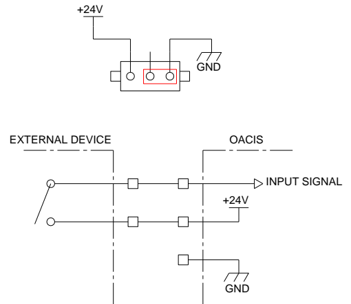
< PNP TYPE INPUT JUMPER SETTING >
