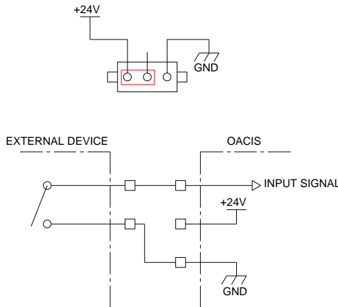
< NPN TYPE INPUT JUMPER SETTING >
